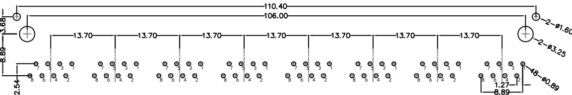
RECOMMENDED PCB LAYOUT VIEWED FROM COMPONENT SIDE
